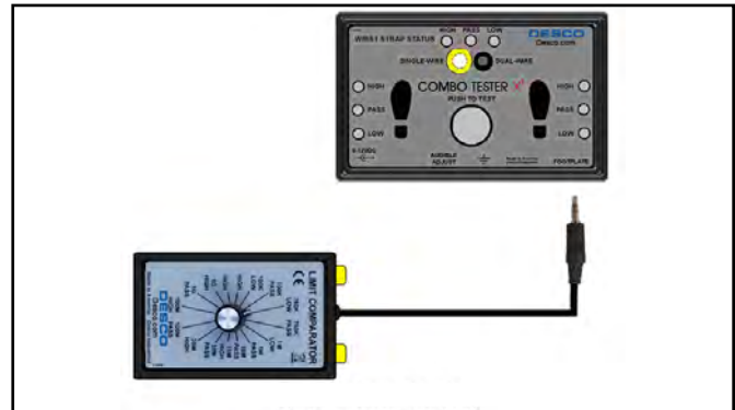
Figure 3. Footwear Test Setup
