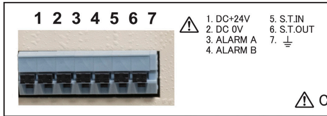
Figure 3. Terminal block
