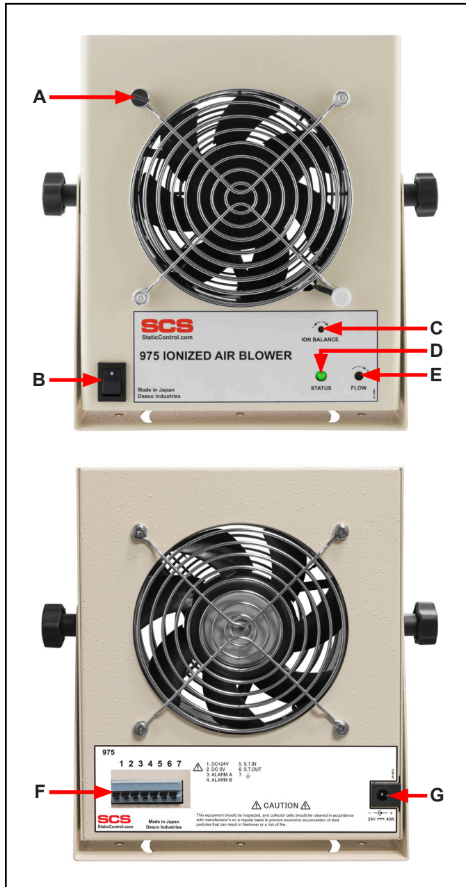
Figure 2. 975 Ionized Air Blower features and components
