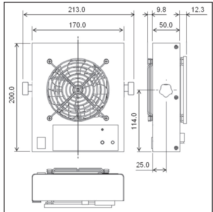
Figure 11. General dimensions of the 975 Ionized Air Blower (mm)
