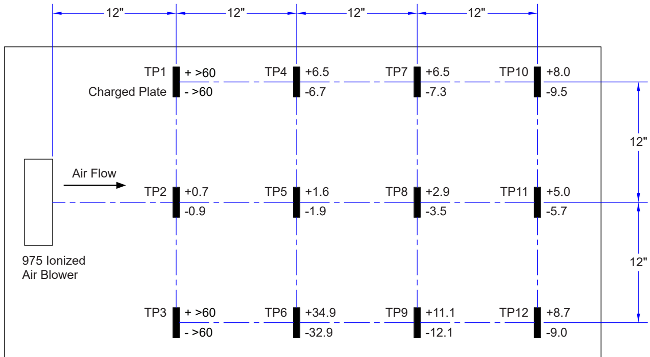
Figure 11. Neutralization (discharge) times in seconds
