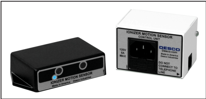
Figure 17. Desco 60509 Ionizer Motion Sensor
