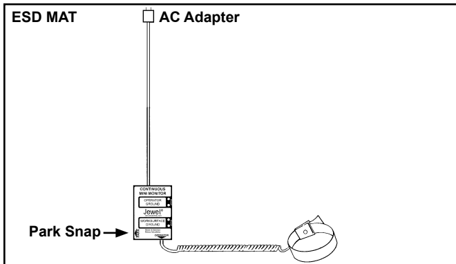
Figure 4. Operating the Jewel® Workstation Continuous Mini Monitor.
