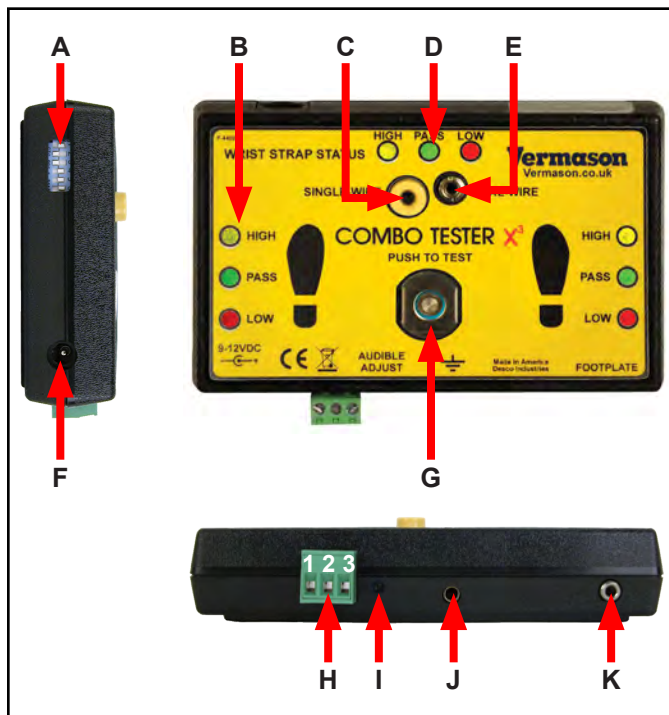
Figure 2. Vermason Combo Tester X3 features and components
