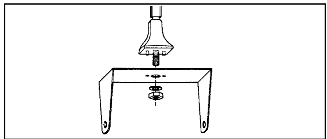
Figure 5. Installing Chargebuster Jr. to Ionizer Mounting Arm
