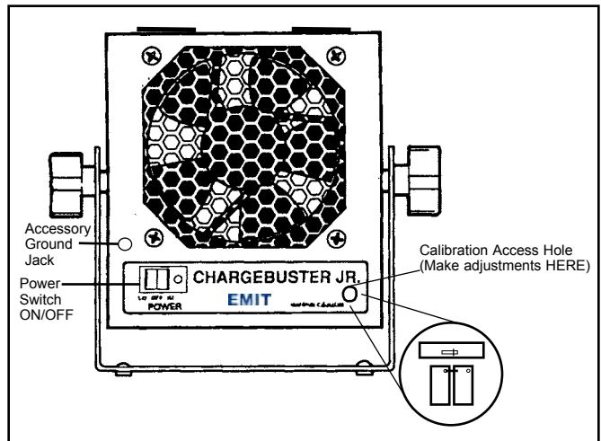
Figure 8. Calibration and position of charged plate for calibration
