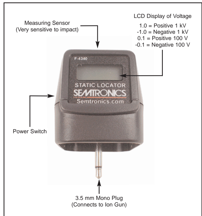
Figure 2. Semtronics Static Locator Features and Components
