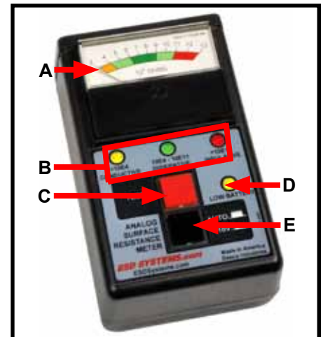
Figure 2. Analog Surface Resistance Meter features and components
