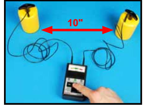
Figure 4. Using the test leads and two 5 pound electrodes to measure RTT of worksurfaces (place electrodes about 3 feet apart for flooring)
