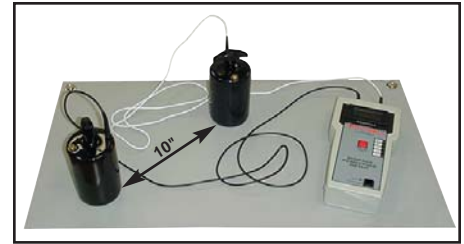
Figure 4. Setting up for RTT testing.
