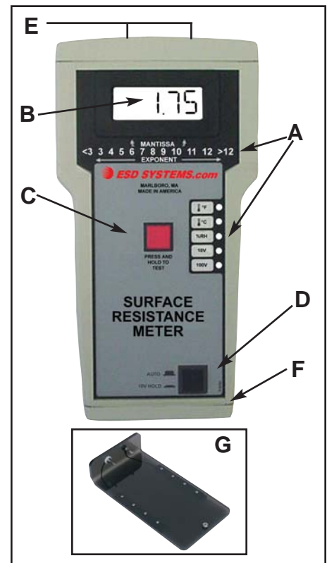
Figure 2. Features of the Surface Resistance Meter
