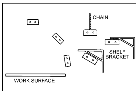
Figure 3. Mounting alternatives relative to the bench top
