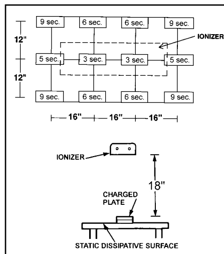
Figure 7. Decay time in seconds from 1000 volts to 100 volts on a 6" x 6" charged plate per ESD-S3.1.
