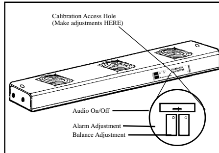
Figure 8. Calibration and position of charged plate for calibration.
