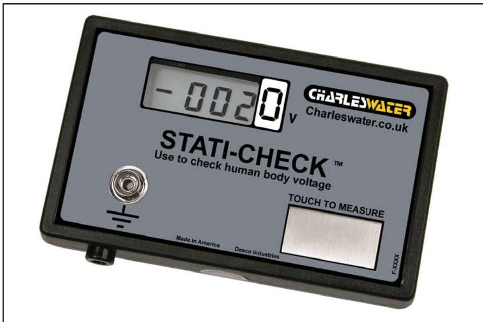
Figure 1. Charleswater 99137 Stati-Check™ Personnel Static Charge Visualiser
