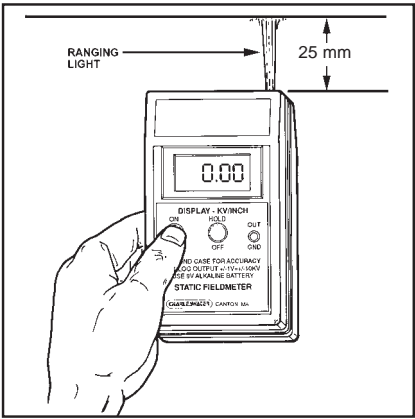
Figure 2. Zeroing the meter
