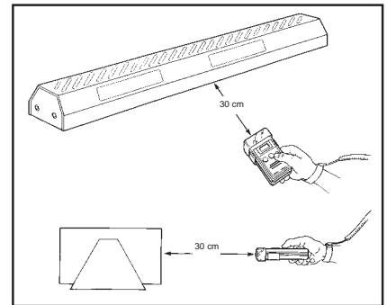
Figure 4. Auditing ionisation equipment with the Digital Fieldmeter and the Ionisation Test Kit.
