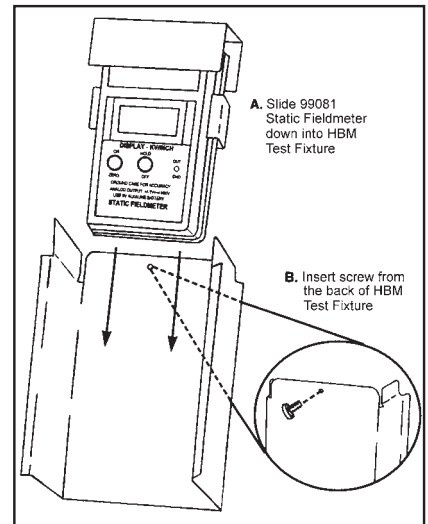
Figure 6. Installing HBM Test Fixture on 99081 Digital Field Meter
