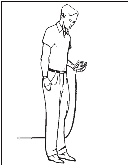
Figure 7. Using the HBM Test Fixture to measure charges on the body.
